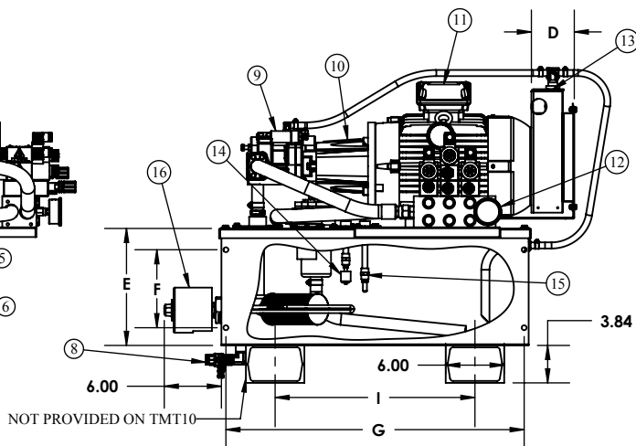
TMT20 - 10HPC3 - PCP8-3K-2AK3 - HE90H W/ D03 VALVES, FLOAT / TEMP SWITCHES
