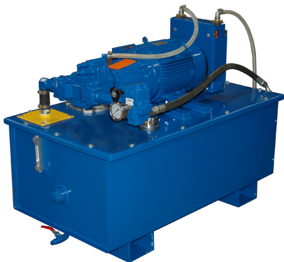
TMT70 SHOWN WITH OPTIONAL HE165H CASE COOLER
