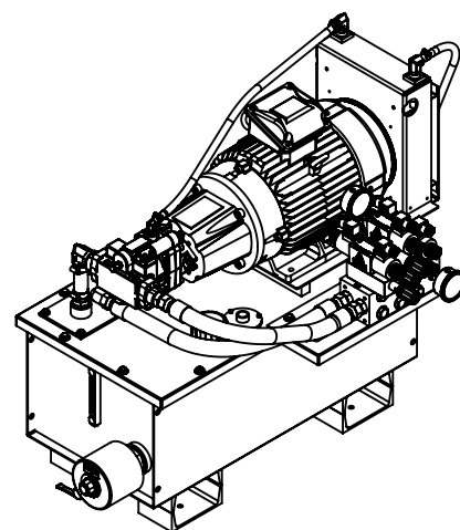
TMT20 - 10HPC3 - PCP8-3K-2AK3 - HE90H W/ D03 VALVES, FLOAT / TEMP SWITCHES
