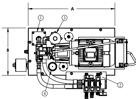
TMT70 SHOWN WITH OPTIONAL HE165H CASE COOLER
